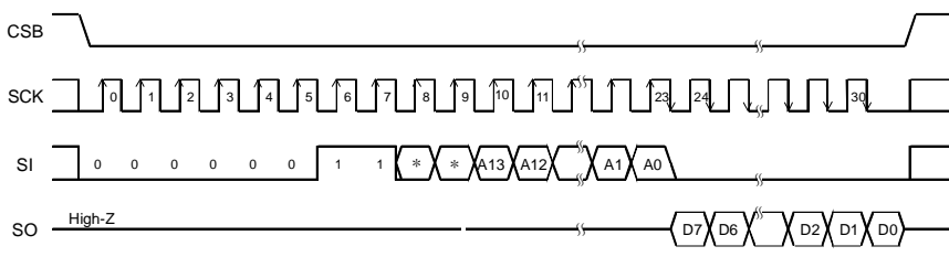
Figure 37. Read command
