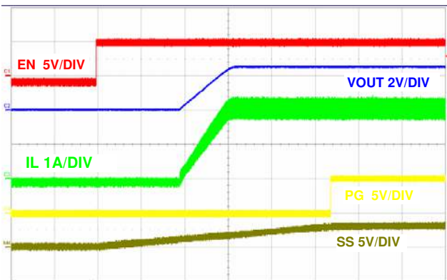
FIGURE 16. SOFT-START AT FULL LOAD (2ms/DIV)
