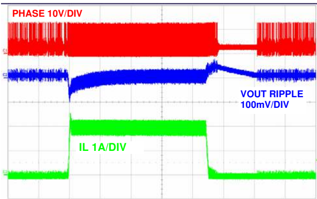
FIGURE 14. LOAD TRANSIENT (200 \mu\text{s} /DIV)
