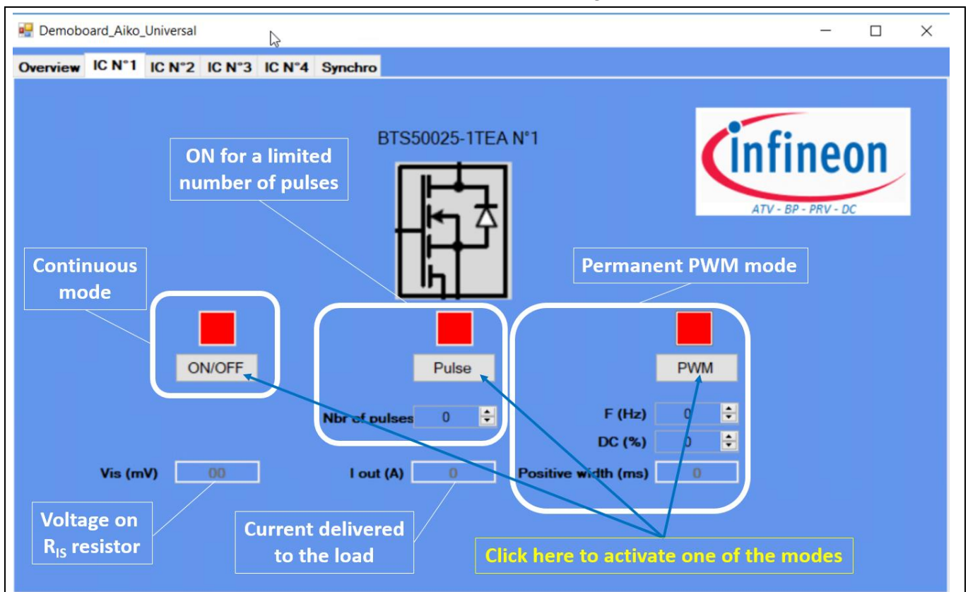
Figure 7 Control Modes
