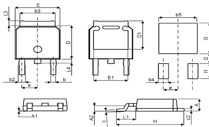
TO-252, (TO-252)
