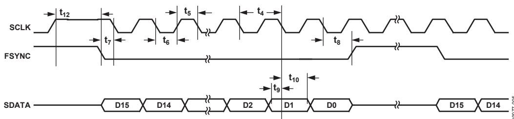
Figure 4. Serial Timing
