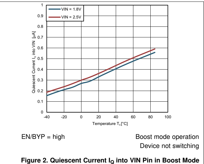
Figure 2. Quiescent Current I_Q into VIN Pin in Boost Mode
