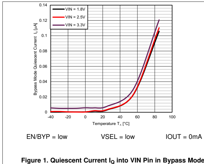
Figure 1. Quiescent Current I_Q into VIN Pin in Bypass Mode
