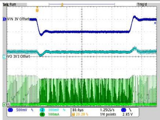
V_{IN} = 2.5V/3V L = 3.3\mu H C_{OUT} = 22 \mu F V_{OUT} = 3.3V V_{SEL} = GND Load = 100Ω
