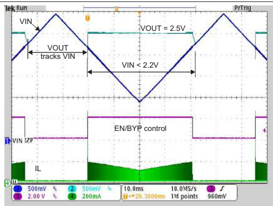
V_{IN} = 0.9V \text{ to } 3V V_{SEL} = \text{Open} I_{LOAD} = 5mA V_{OUT} = 2.5V EN/BYP externally controlled Bypass / Boost mode operation
