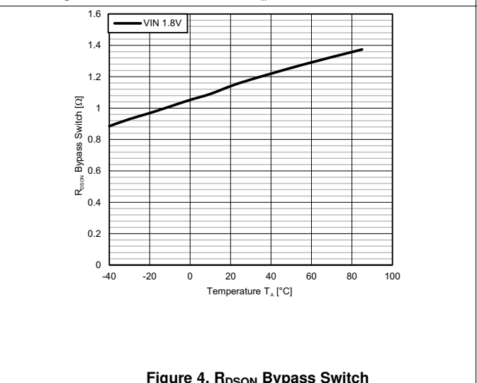
Figure 4. R_{DS(on)} Bypass Switch
