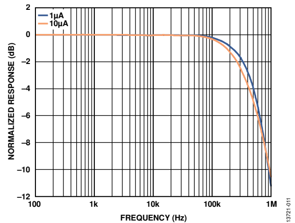
Figure 9. Bandwidth/Peaking
