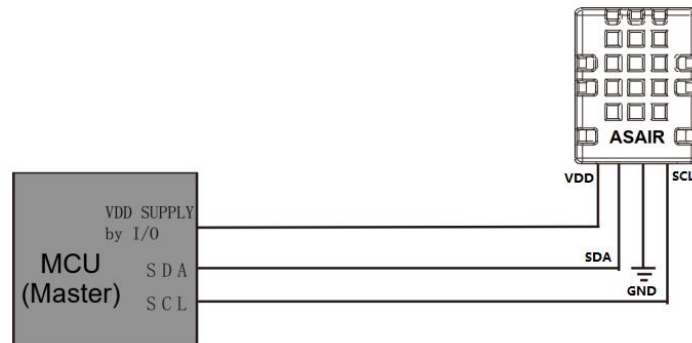
Figure 8. Typical application circuit
