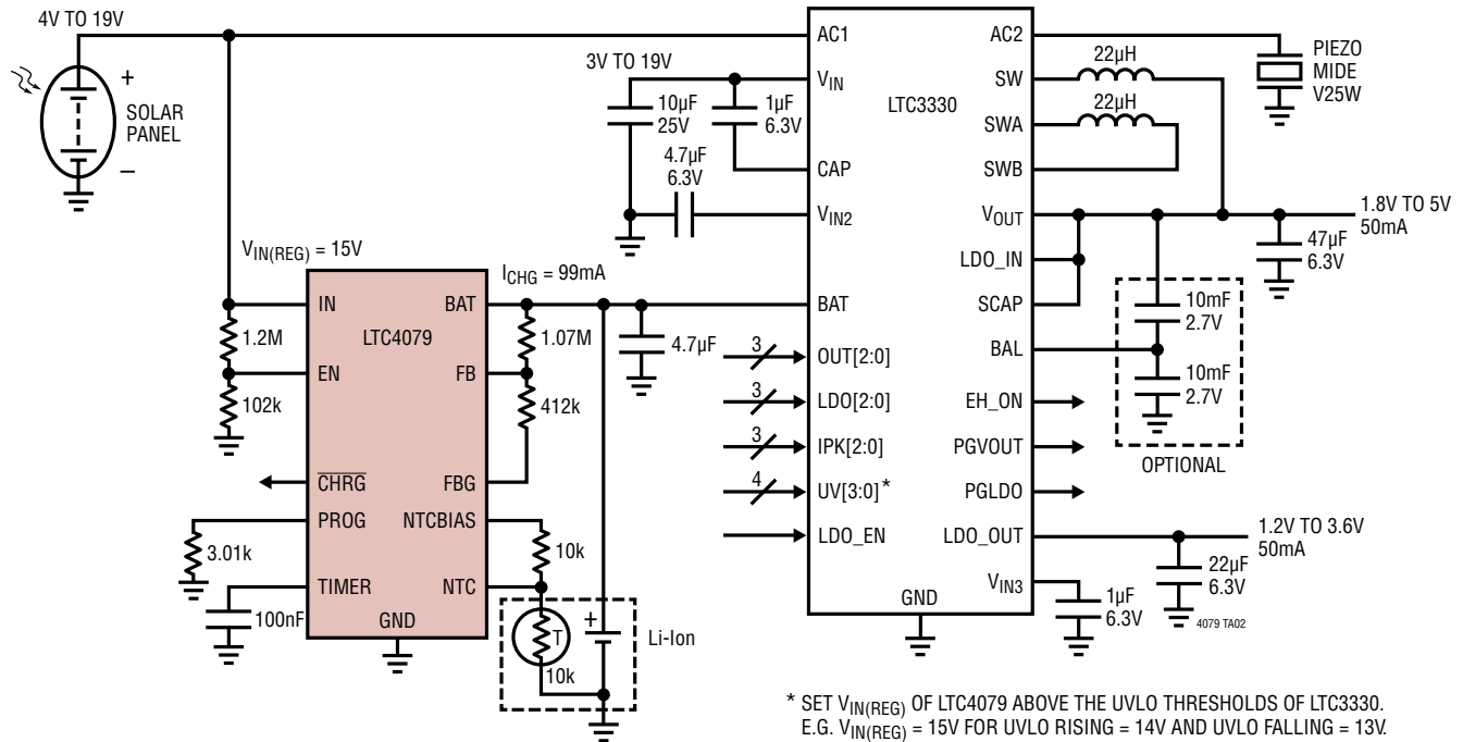
Energy Harvesting Charger with Buck, Buck-Boost and LDO Supplies
