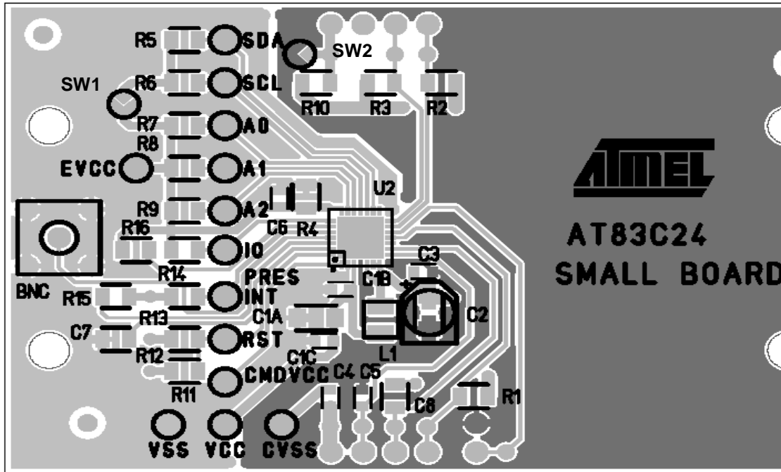
Figure 1-2. Component Side
