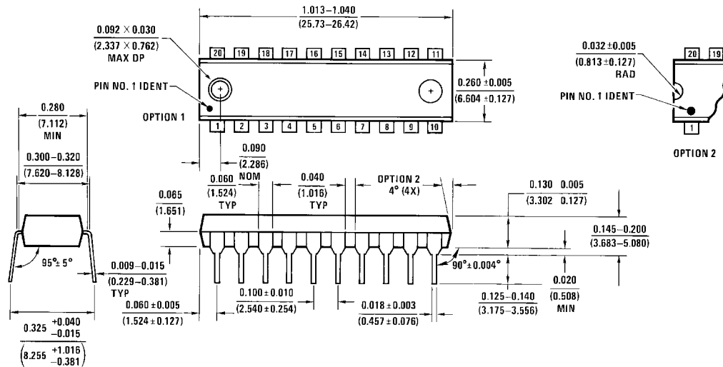
20-Lead Molded DIP (N) Package Number N20A
