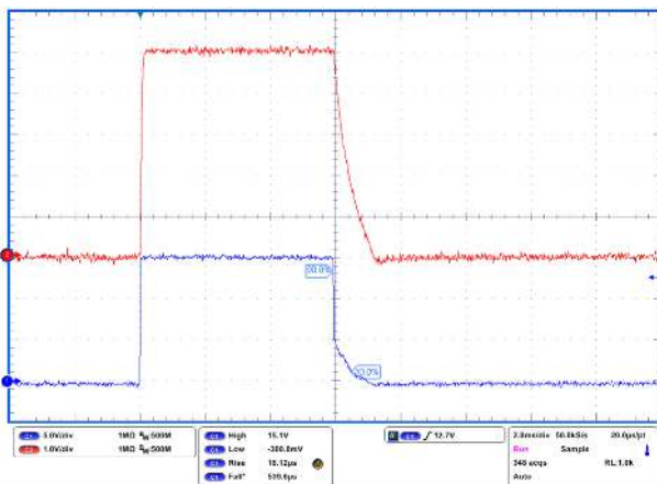
Figure 22. Turn-on time ( V_{OUT} = 5\text{ V} )
