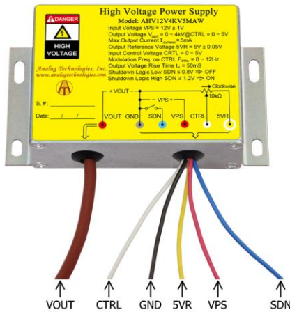
Figure 2. The Connecting Lead Wires of AHV12V4KV5MAW
