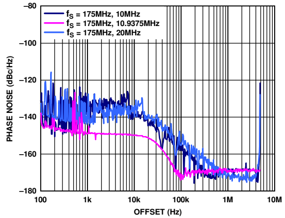
Figure 17. Phase Noise
