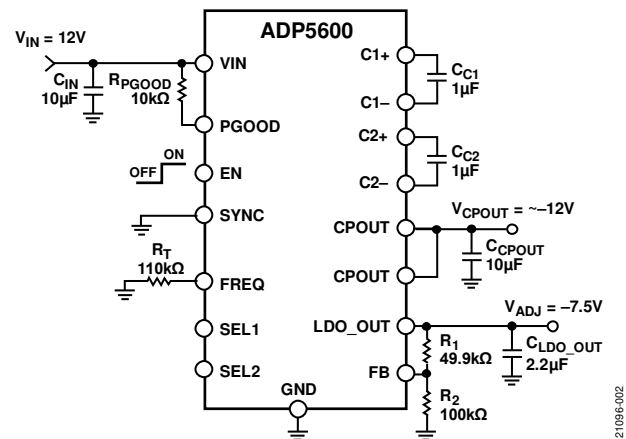
Figure 2. Adjustable Output Voltage, V_{ADJ} = -7.5\text{ V}
