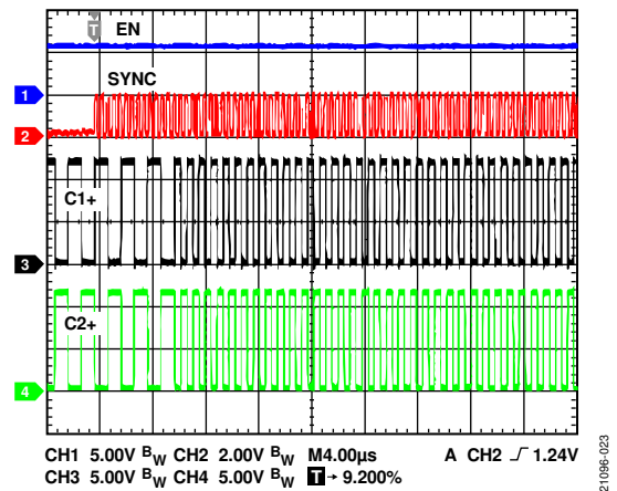
Figure 23. Oscillator Frequency ( f_{osc} ) Transition, R_T = 110\text{ k}\Omega to f_{SYNC} = 2.2\text{ MHz}
