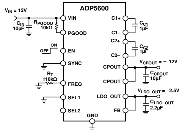
Figure 1. Fixed Output Voltage, V_{LDO\_OUT} = -2.5\text{ V}
