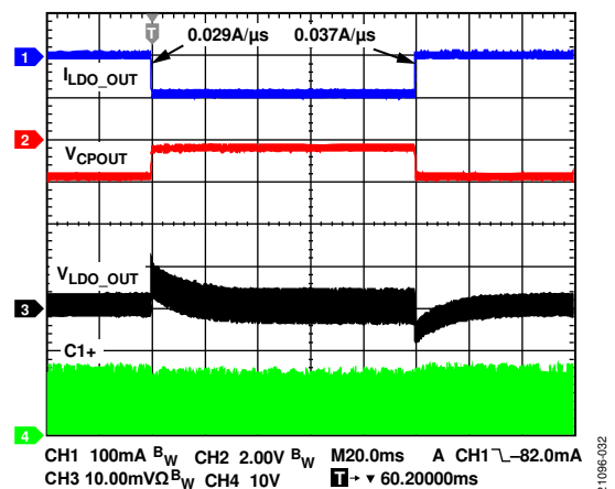
Figure 24. Load Transient Response, I_{LDO\_OUT} = -1\text{ mA} to -100\text{ mA}
