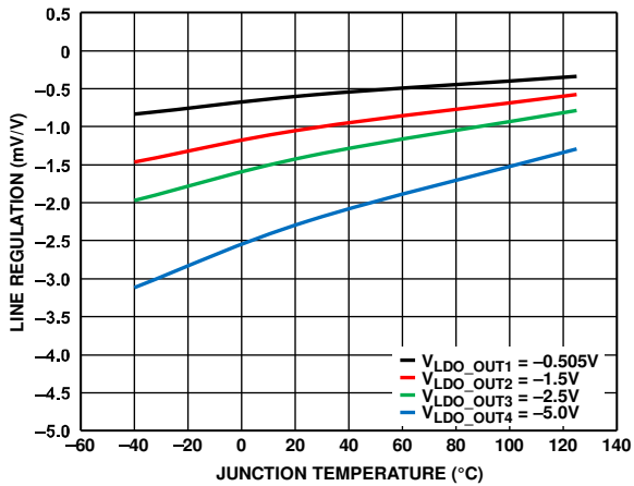
Figure 11. LDO Line Regulation vs. Junction Temperature ( T_J )
