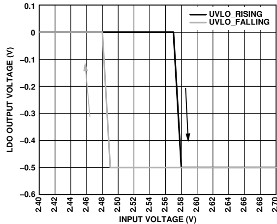
Figure 54. UVLO Threshold
