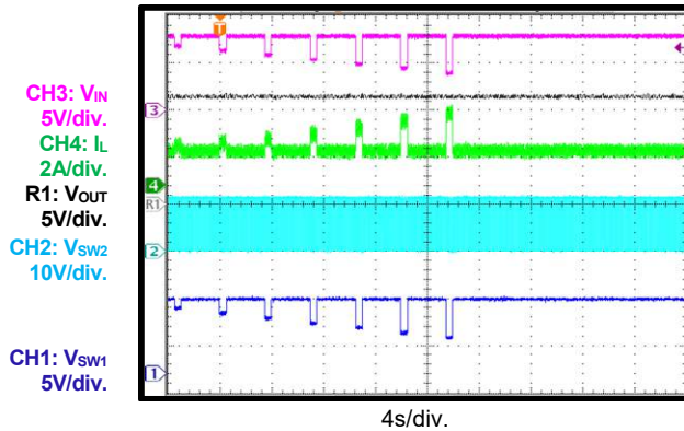
Reset Behavior I_{OUT} = 1A
