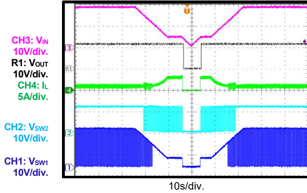
V_{IN} Ramps Down and Up I_{OUT} = 1A
