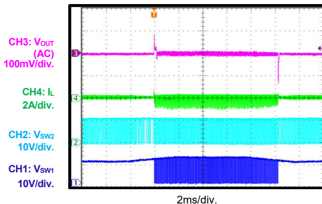
Mode Transient between Boost and Buck-Boost
