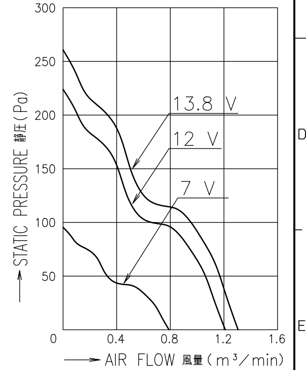
PERFORMANCE CURVES
