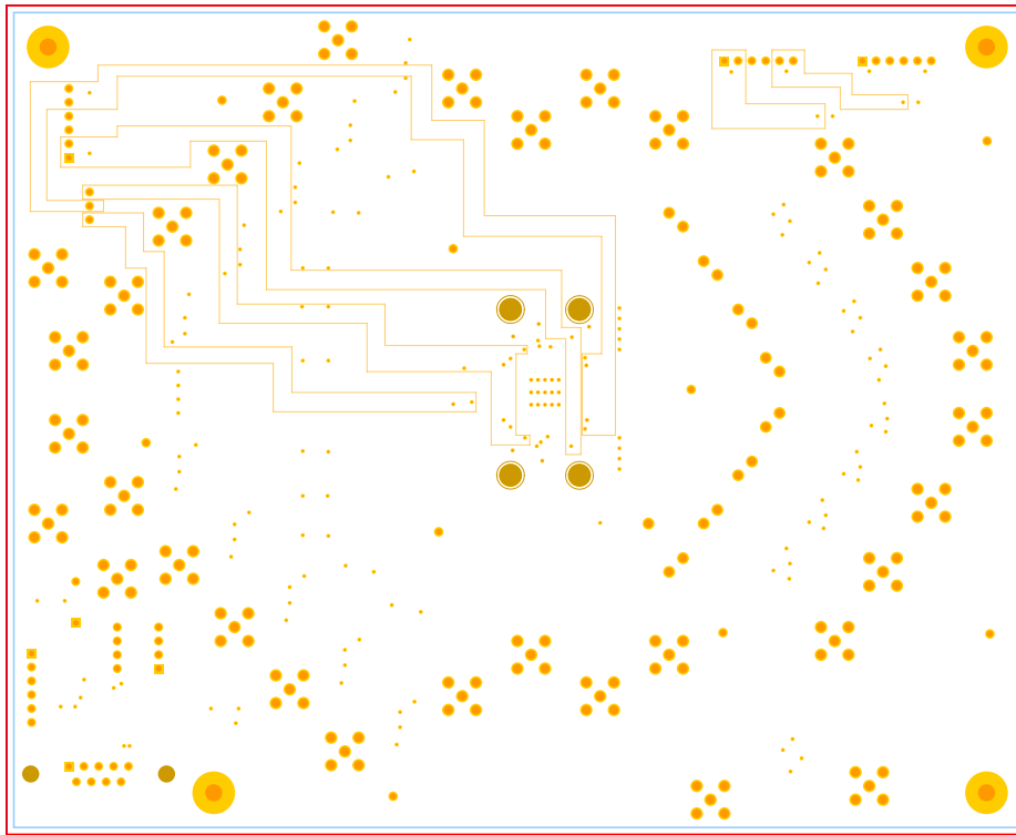
Figure 8. Power Plane 2
