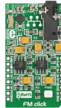
FM Click Features Si4703 IC and functions as a FM radio tuner. Supports worldwide FM band (76-108 MHz).
