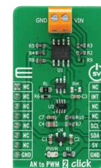
AN to PWM 2 Click Features the LTC6992CS6, a silicon oscillator from Analog Devices.
