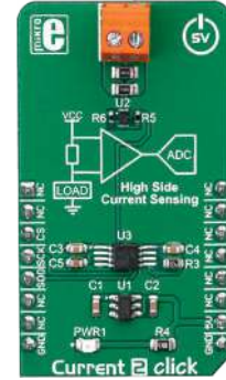
Current 2 Click Equipped with an integrated transimpedance amplifying circuit.
