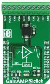
GainAMP 2 Click A 6-channel programmable gain amplifier. Amplifies up to 32x, in eight discrete steps.
