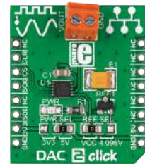
DAC 2 Click Carries LTC2601CDD, a 16-bit digital-to-analog converter from Linear Technology.
