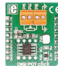
DIGI POT Click Carries MCP416 single-channel 8-bit resolution [256 wiper steps] digital potentiometer.
