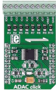
ADAC Click It's an 8-channel 12-bit ADC, DAC and GPIO. With AD5593R configurable ADC/DAC.
