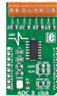
ADC 3 Click With Microchip's MCP3428 16-bit multichannel analog-to-digital converter.
