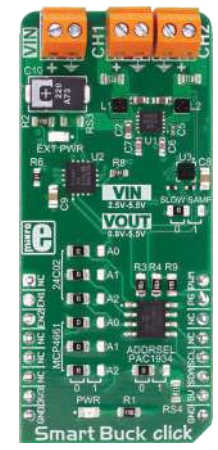
Smart Buck Click The MIC2230, a dual synchronous step-down DC/DC regulator.
