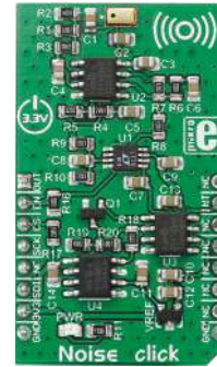
Noise Click With noise detecting circuitry. Enables you to set a noise detection threshold.
