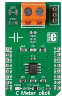
C Meter Click Circuitry for measuring the value of capacitors. Based on NE-555 timer/square-wave generator.
