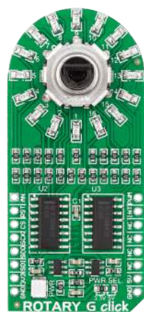
ROTARY G Click
