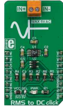
RMS to DC Click With the LTC1968, converter IC, which outputs an analog voltage depending on the RMS value of the input signal.
