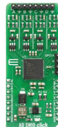
AD-SWIO Click The AD74412R a quad-channel software configurable input/output solution.
