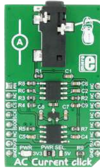
AC Current Click Measure alternating currents up to 30A. MCP3201 ADC converter and MCP607 CMOS Op Amp.
