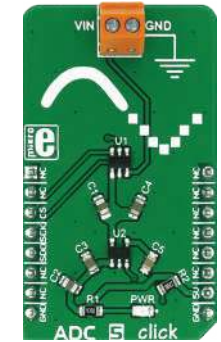
ADC 5 Click With a low power, single channel 12-bit CMOS analog to digital converter.
