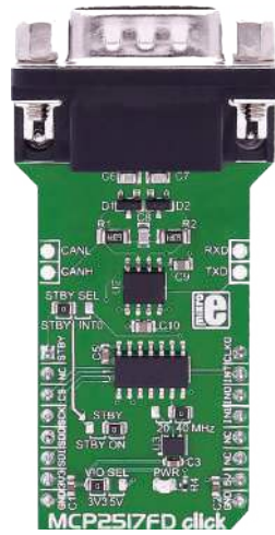
MCP2517FD Click With MCP2517FD CAN FD controller and ATA6563 high-speed CAN transceiver. MSRP - $25 00 MIKROE-2379
