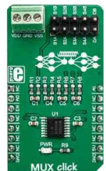
MUX Click Equipped with the MUX509, a precise analog multiplexing IC.
