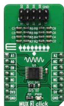
MUX 3 Click Based around the TMUX1208 module, a 5-V Bidirectional 8:1, 1-Channel Multiplexer.
