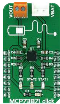
MCP73871 Click Integrated solution for system power delivery and Li-Po/Li-Ion battery charge management.
