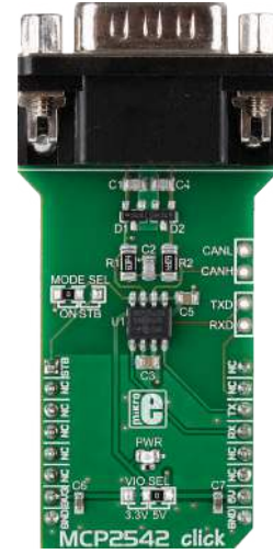
MCP2542 Click Microchip's CAN FD Transceiver with Wake-Up Pattern. Compliant with CAN 2.0 and CAN FD. MSRP - $20 00 MIKROE-2289
