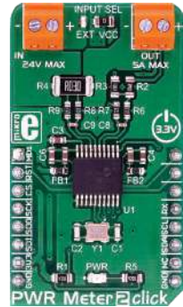
PWR Meter 2 Click Measuring and monitoring voltage up to 24V and current up to 5A. It carries the MCP3910 module.
