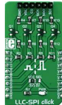
LLC-SPI Click Used as the level converter for logic signals. It is perfectly suited for SPI communication. MSRP - $9 00 MIKROE-3298
