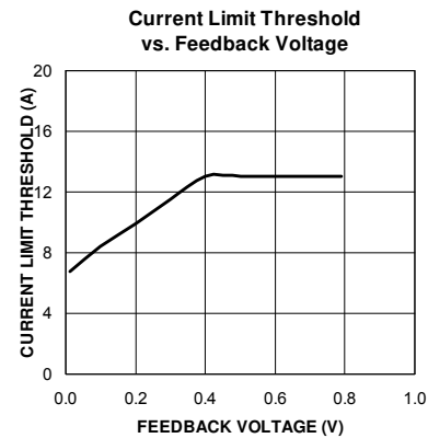
Figure 5. MIC26603 Current Limit Foldback Characteristic
