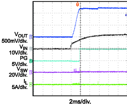
Startup through VIN PFM, I_{OUT}=0A
