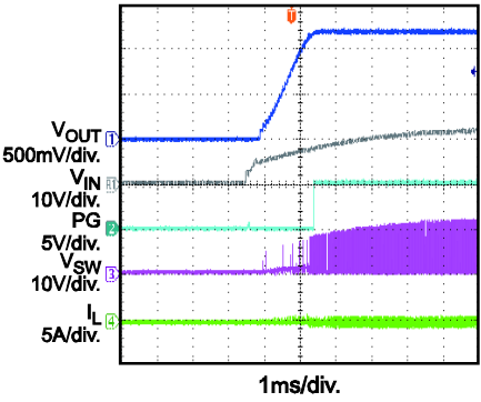
Startup through VIN Force PWM, I_{OUT}=0A
