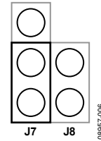
Figure 6. Jumper Settings (J7 and J8) for Jack Detection (Low Signal Detected)
