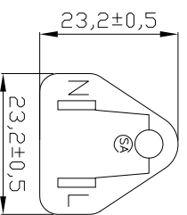
PLUG TYPE
