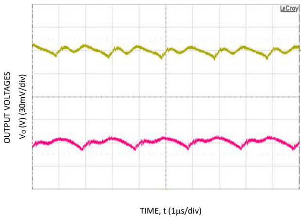
Figure 9. Typical output ripple and noise ( C_0 = 2 \times 4.7nF + 2 \times 47\mu F ceramic, V_{IN} = 12V , I_o = I_{o1,max}, I_{o2,max} ).
