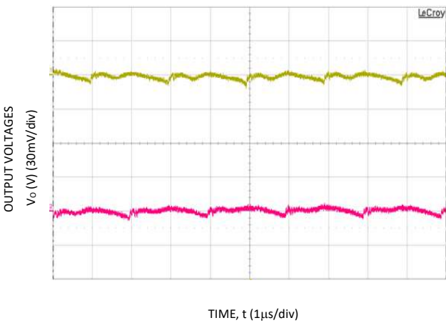
Figure 3. Typical output ripple and noise ( C_0 = 2 \times 4.7\text{nF} + 2 \times 47\text{uF} ceramic, V_{IN} = 12\text{V} , I_o = I_{o1,max}, I_{o2,max} ).
