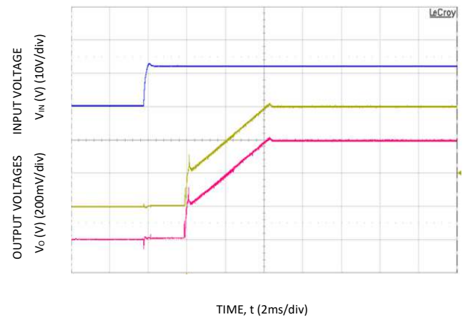
Figure 6. Typical Start-up Using Input Voltage ( V_{IN} = 12\text{V} , I_o = I_{o1,max}, I_{o2,max} ).
