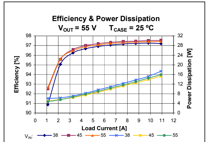
Figure 8 – Total efficiency and power dissipation vs. V_{IN} and I_{OUT} , V_{OUT}=55\text{V} , T_{CASE}=25^{\circ}\text{C}
