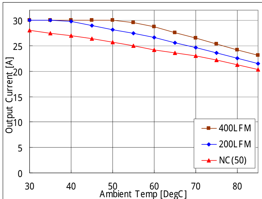
Fig-1.8V-1: Available load current vs. ambient temperature and airflow rates for Vout=1.8V with Vin=12.0V. Maximum component temperature ≤ 120°C
