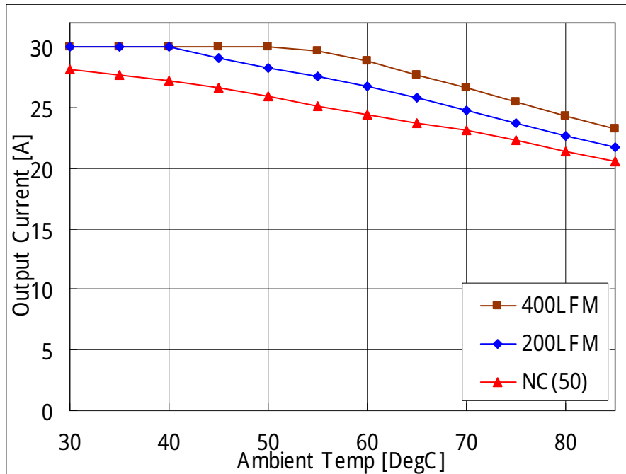
Fig-1.5V-1: Available load current vs. ambient temperature and airflow rates for V_{out}=1.5V with V_{in}=12.0V . Maximum component temperature \leq 120^{\circ}C
