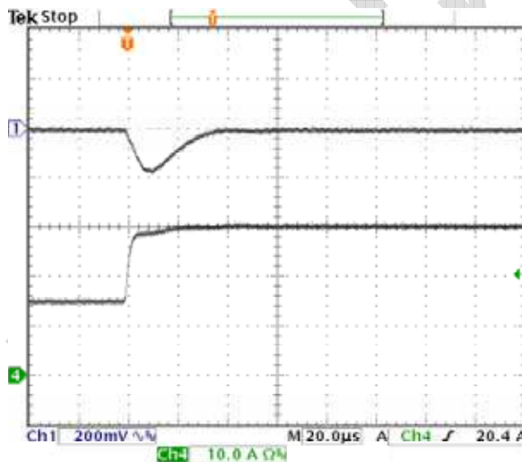
Fig-2.0V-6: Output voltage response for V_{out}=2.0V to positive load current step-change from 15A to 30A with slew rate of 5A/\mu s at V_{in}=12.0V . C_o=47\mu F \times 2 ceramic. Top trace: output voltage (200mV/div.) Bottom trace: load current (10A/div.) Time scale: 20μs/div.
