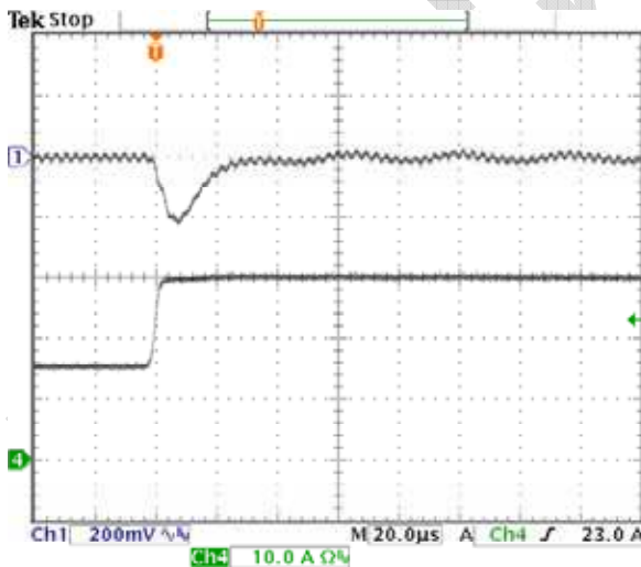
Fig-5.0V-6: Output voltage response for V_{out}=5.0V to positive load current step-change from 15A to 30A with slew rate of 5A/\mu s at V_{in}=12.0V . C_o=47\mu F \times 2 ceramic. Top trace: output voltage (200mV/div.) Bottom trace: load current (10A/div.) Time scale: 20μs/div.
