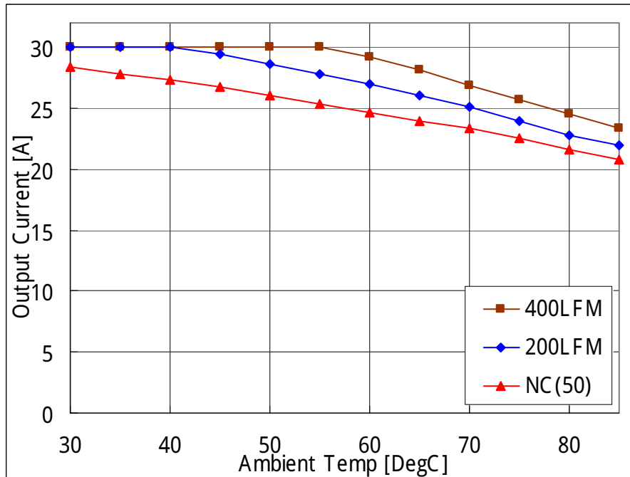
Fig-1.2V-1: Available load current vs. ambient temperature and airflow rates for Vout=1.2V with Vin=12.0V. Maximum component temperature ≤ 120°C
