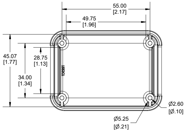
INSIDE BOTTOM
