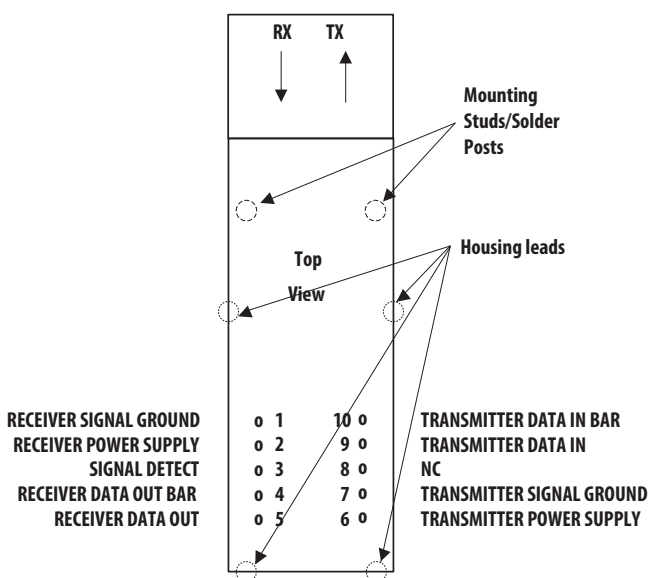
Figure 1: Pinout Diagram
