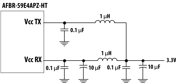
Figure 3: Recommended Power Supply Filter
