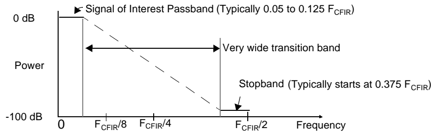
Figure 10. Typical CFIR Specifications
