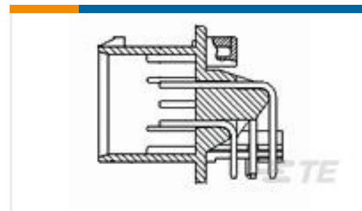
TE Part #776266-5 14POS,PIN DIA 1.3,HDR ASSY,90DEG, COD 5
