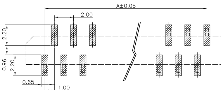
MOUNTING LAYOUT (CONN.MOUNTING SIDE)
