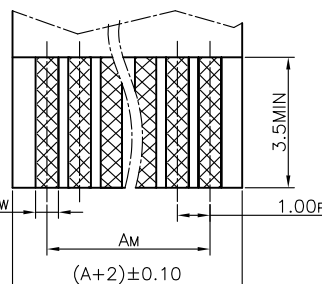
APPLICABLE FPC/FFC
