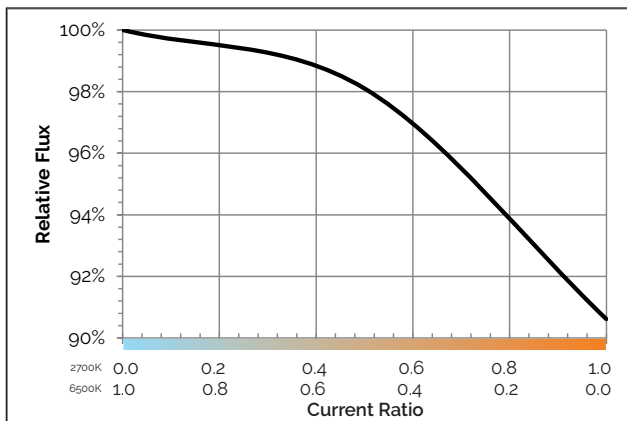
Figure 9: Flux vs. Current Ratio (2700K-6500K)
