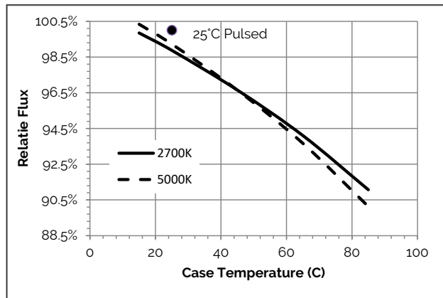
Figure 12: Flux vs Case Temperature (2700K-5000K)
