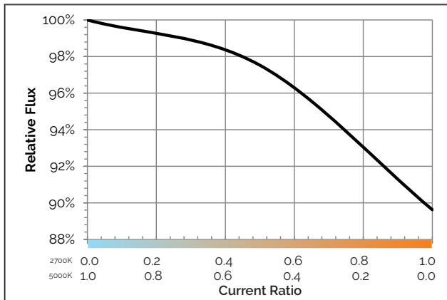
Figure 7: Flux vs. Current Ratio (2700K-5000K)
