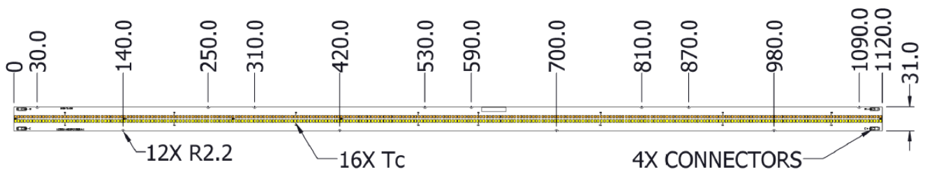
Figure 19: Drawing Overview for 1120mm
