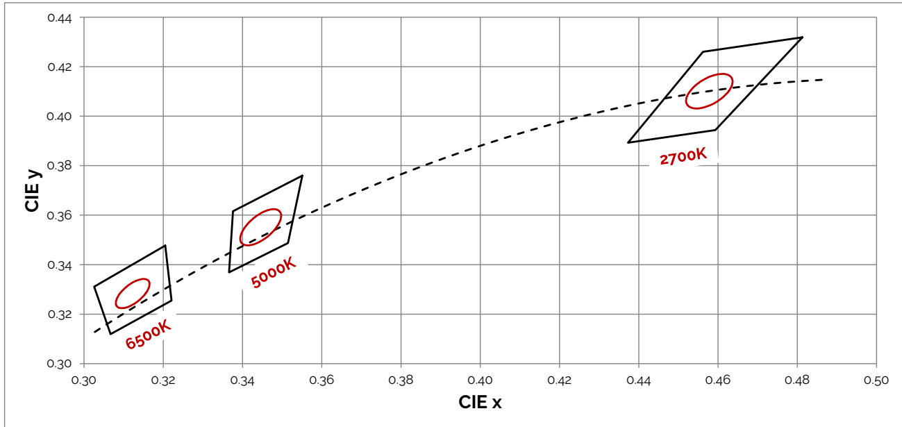
Figure 20: 3 SDCM Color Bins in CIE 1931 xy Color Space
