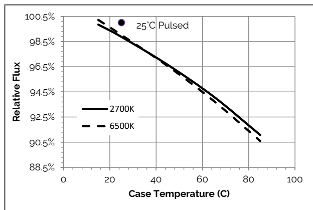
Figure 13: Flux vs Case Temperature (2700K-6500K)
