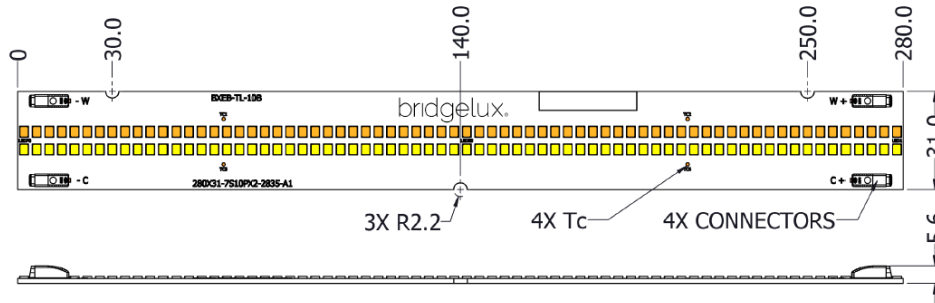
Figure 17: Drawing Overview for 280mm
