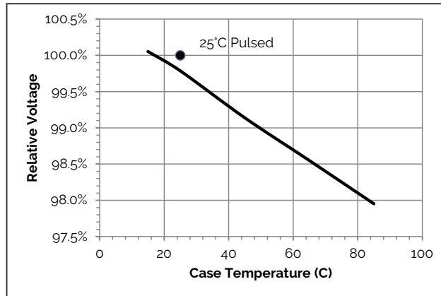
Figure 11: Voltage vs Case Temperature
