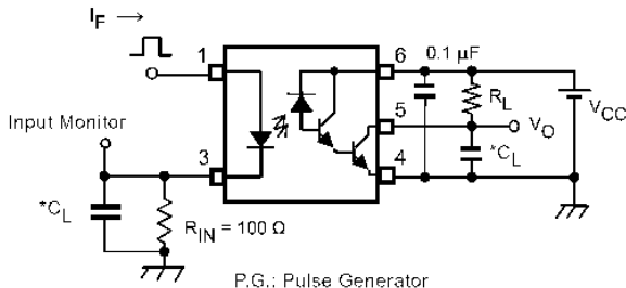
Fig. 12.1.1 Switching Time Test Circuit and Waveform
