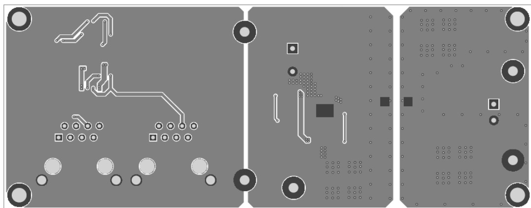
Figure 3: Bottom Layer
