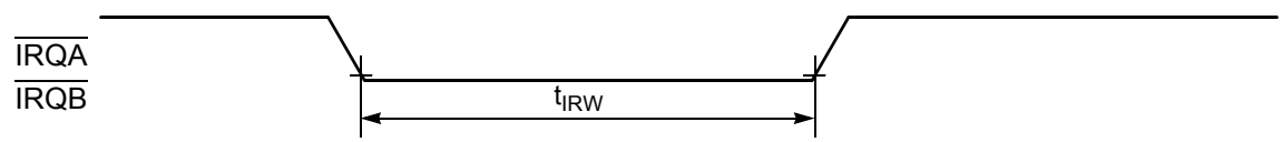
Figure 4-11 External Interrupt Timing (Negative-Edge-Sensitive)
