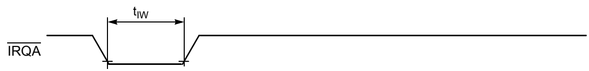
Figure 4-13 Recovery from Stop State Using Asynchronous Interrupt Timing
