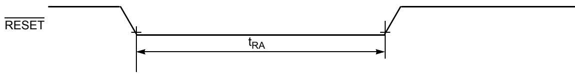
Figure 4-10 Asynchronous Reset Timing
