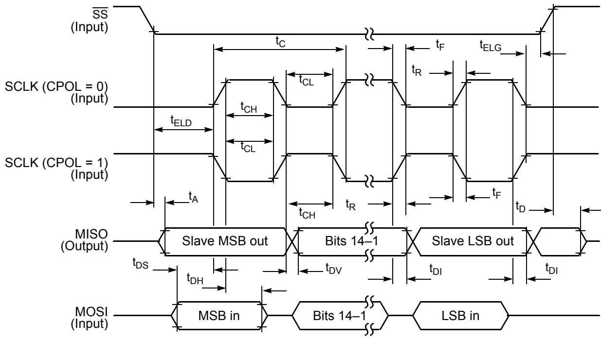
Figure 4-23 SPI Slave Timing (CPHA = 0)
