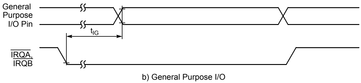
Figure 4-12 External Level-Sensitive Interrupt Timing
