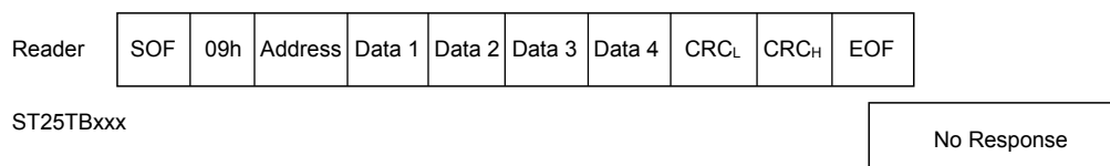
Figure 41. Write_block frame exchange between reader and ST25TB02K
