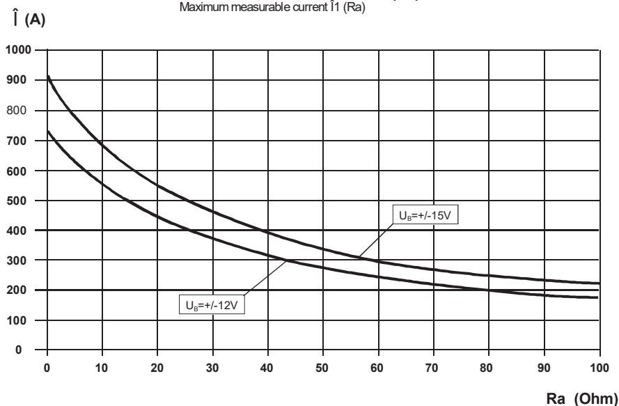
Maximal meßbarer Strom \hat{I}_1 ( R_a ) Maximum measurable current \hat{I}_1 ( R_a )
