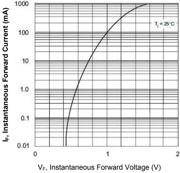
Figure 1. Forward Characteristics
