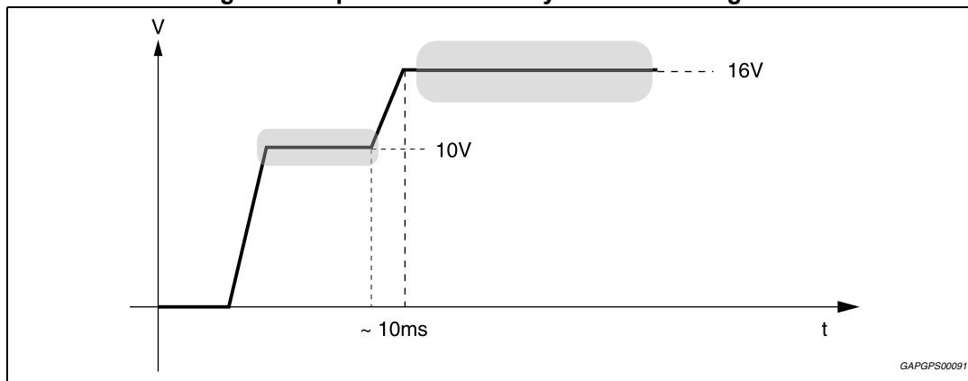
Figure 35. Upwards fast battery transitions diagram
