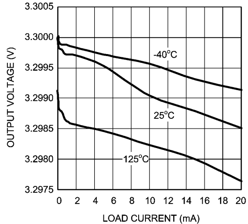
Load Regulation
