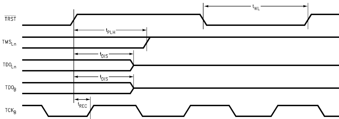
Figure 7. Reset Waveforms
