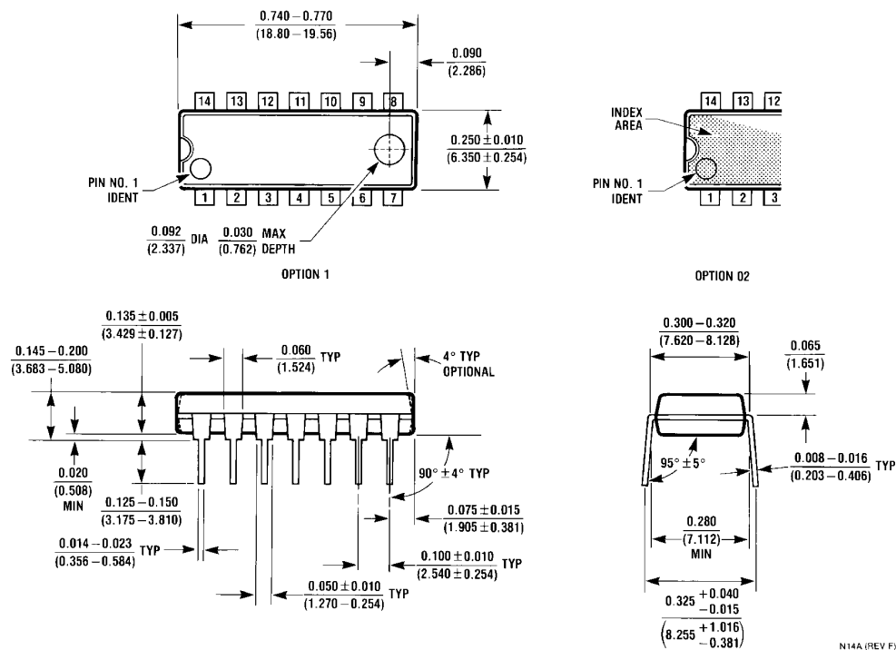
14-Pin Molded Dual-In-Line Package Order Number LMC6064AIN or LMC6064IN NS Package Number N14A
