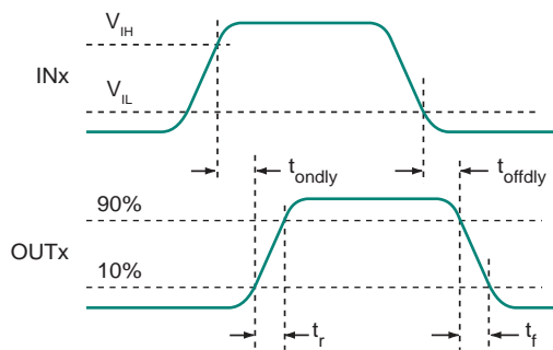
Non-Inverting Driver Waveforms
