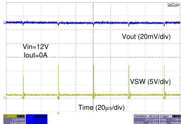
Figure 15. Static Load Ripple at Light-Load
