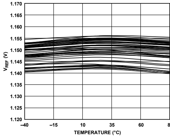
Figure 41. Change in VREF Pin Voltage vs. Temperature for 45 Devices
