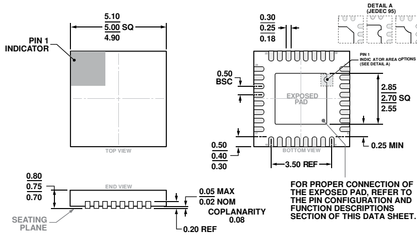
Figure 77. 32-Lead Lead Frame Chip Scale Package [LFCSP] 5 mm × 5 mm Body and 0.75 mm Package Height (CP-32-21) Dimensions shown in millimeters
