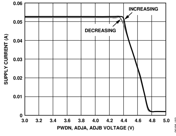
Figure 49. Supply Current vs. V_{PWDN} , V_{ADJA} , V_{ADJB}
