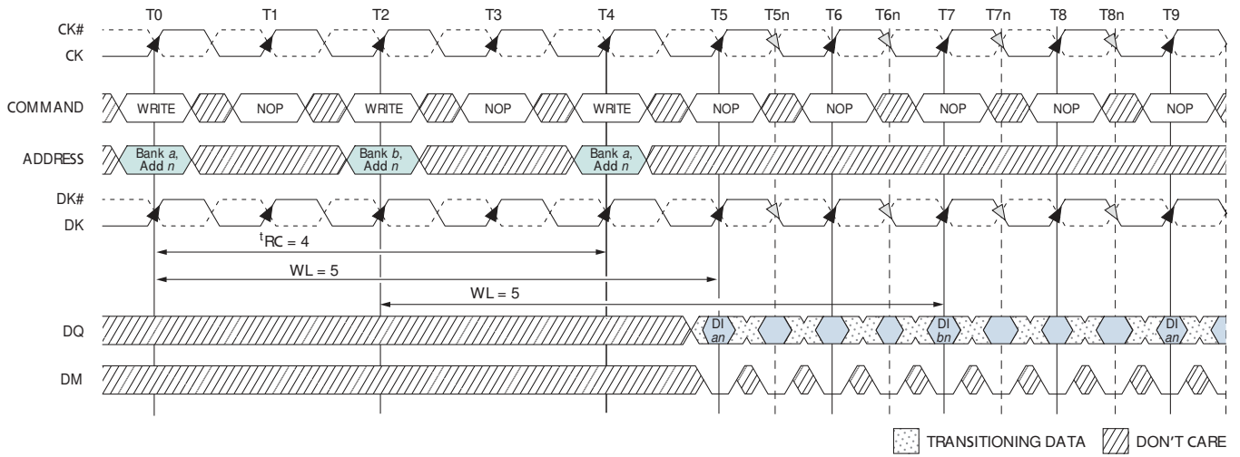
Figure 19: Consecutive WRITE-to-WRITE
