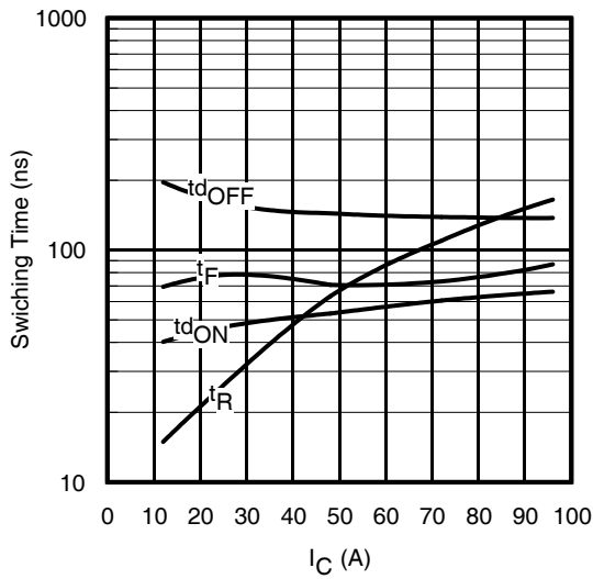
Fig. 14 - Typ. Switching Time vs. I_C T_J = 175^\circ C ; L = 210\mu H ; V_{CE} = 400V , R_G = 10\Omega ; V_{GE} = 15V
