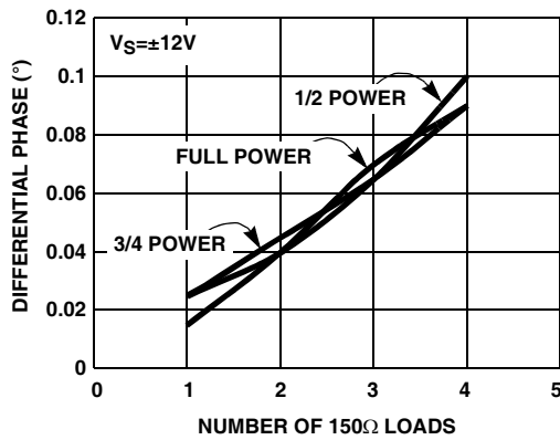
FIGURE 39. DIFFERENTIAL PHASE
