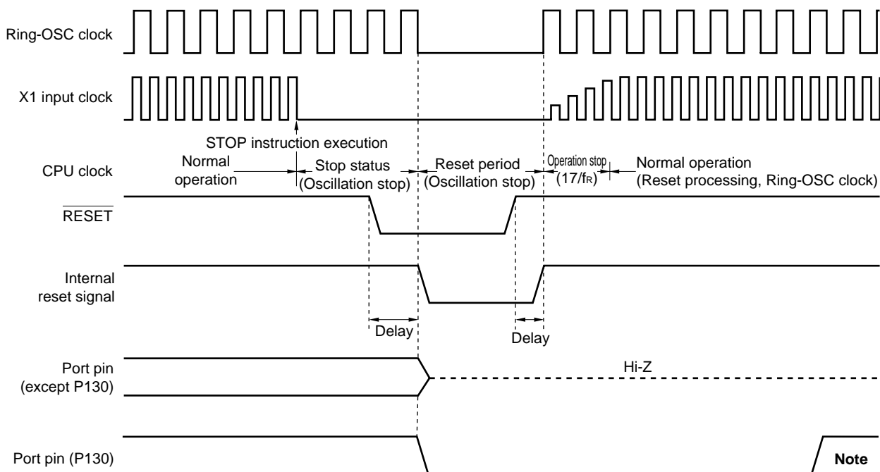
Figure 16-4. Timing of Reset in STOP Mode by RESET Input
