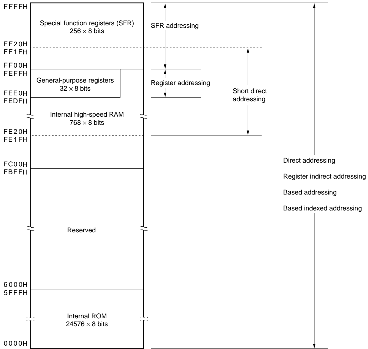
Figure 3-7. Correspondence Between Data Memory and Addressing (ⓂPD780103)
