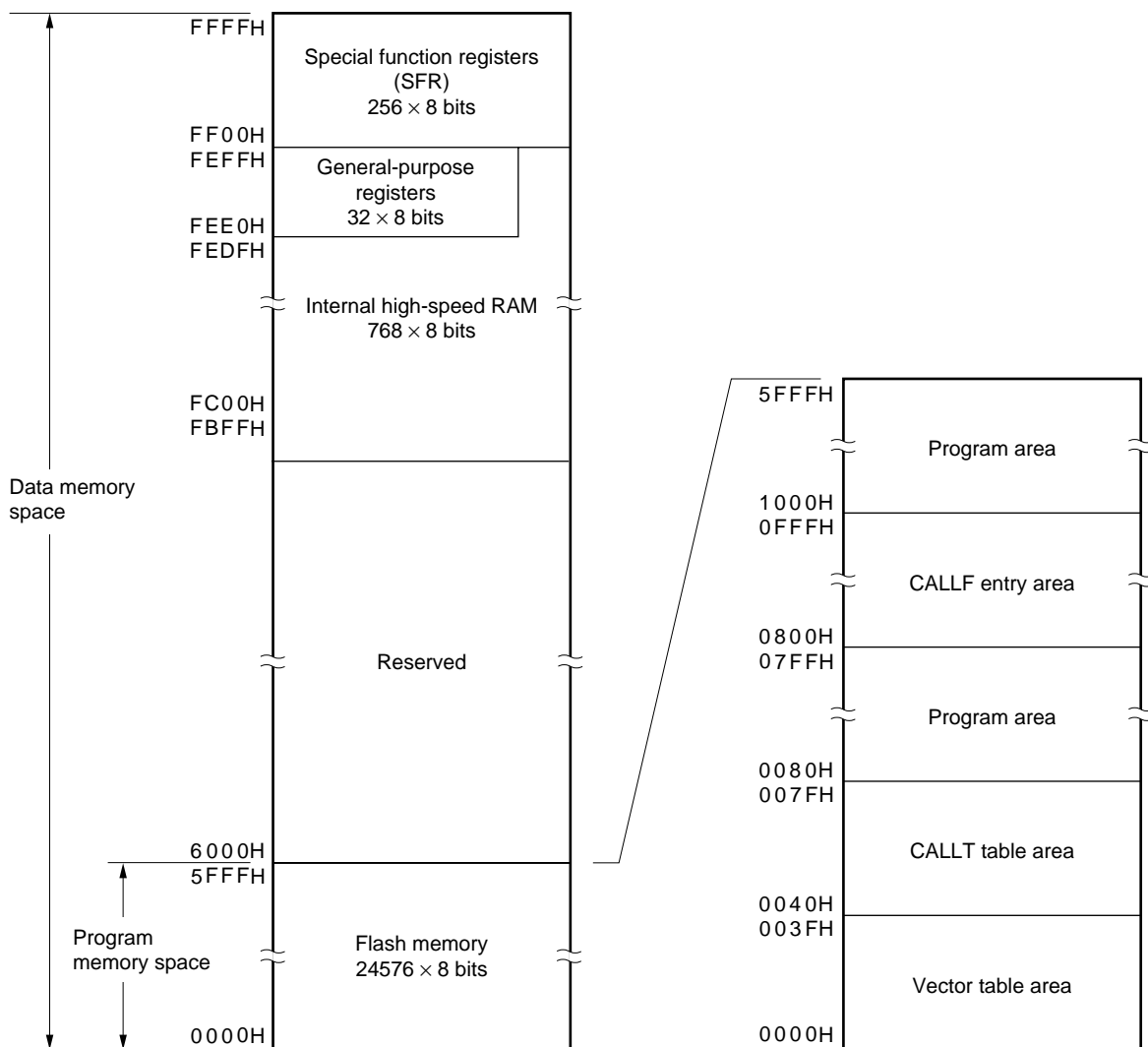
Figure 3-4. Memory Map (αPD78F0103)
