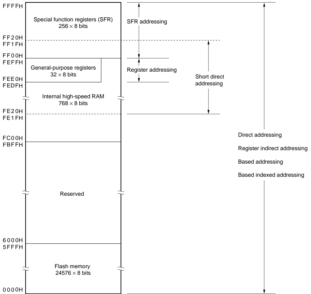
Figure 3-8. Correspondence Between Data Memory and Addressing (ⓂPD78F0103)
