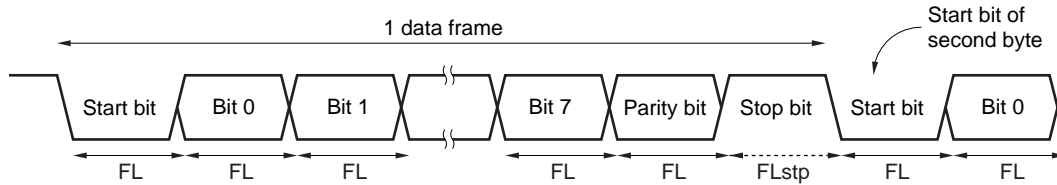
Figure 12-27. Data Frame Length During Continuous Transmission
