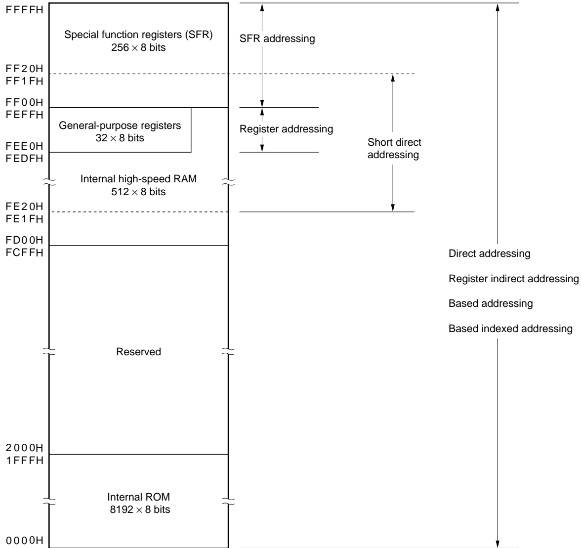
Figure 3-5. Correspondence Between Data Memory and Addressing (≈PD780101)
