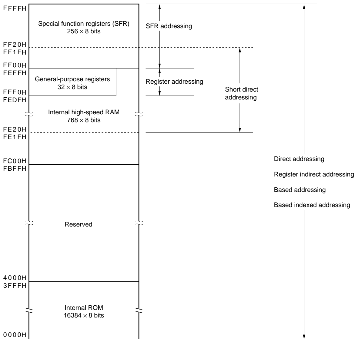
Figure 3-6. Correspondence Between Data Memory and Addressing (PD780102)
