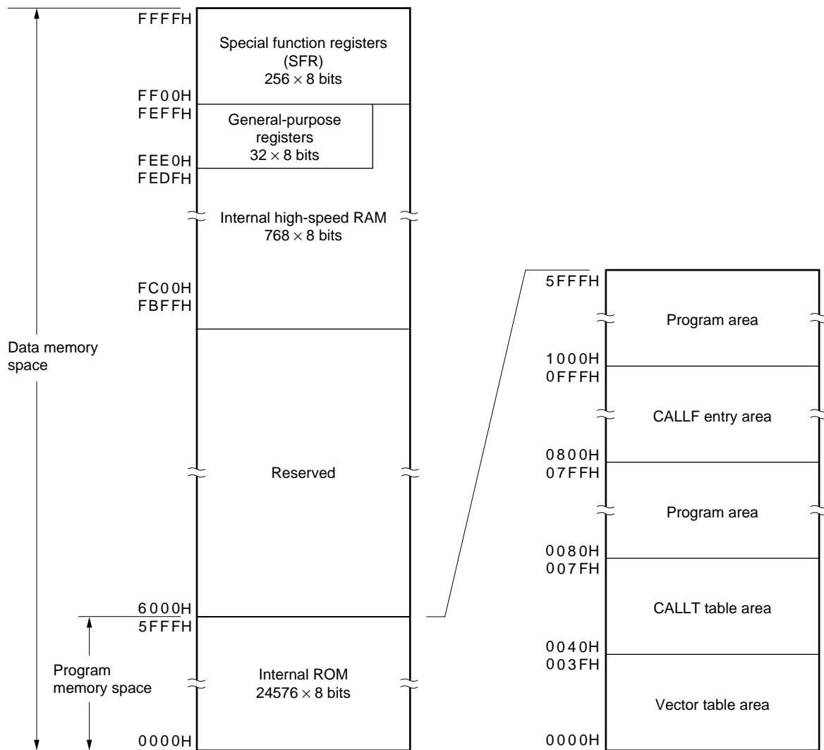
Figure 3-3. Memory Map (PD780103)
