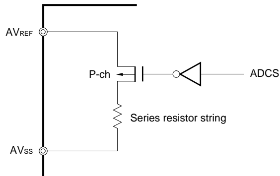
Figure 10-2. Circuit Configuration of Series Resistor String
