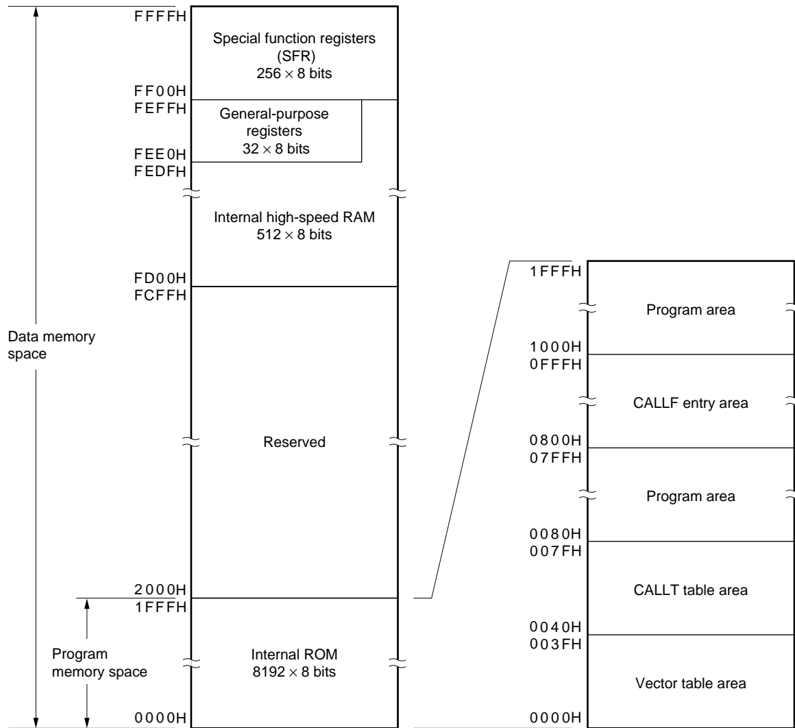
Figure 3-1. Memory Map (PD780101)
