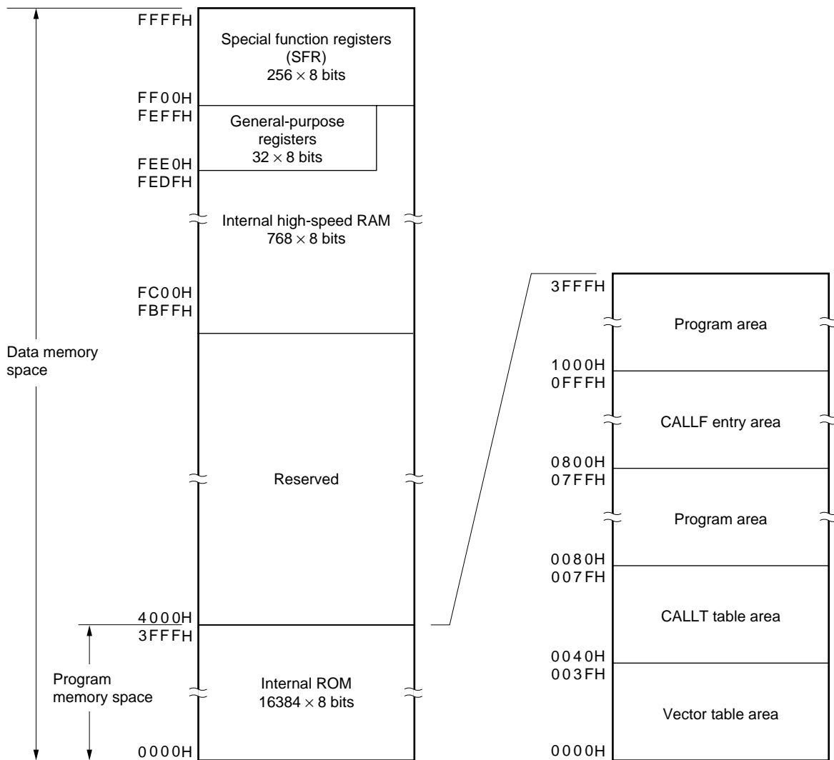
Figure 3-2. Memory Map (M PD780102 )
