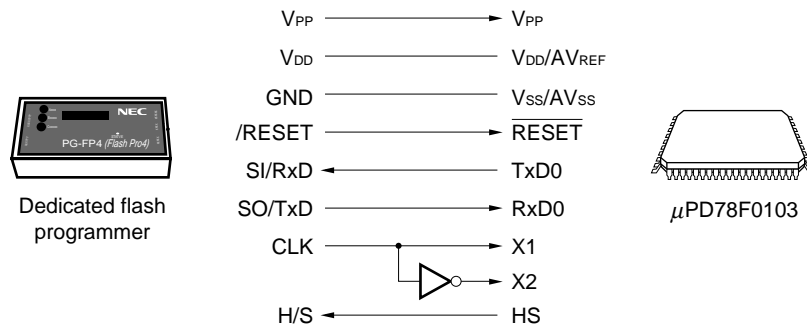
Figure 21-11. Communication with Dedicated Flash Programmer (UART0 + HS)
