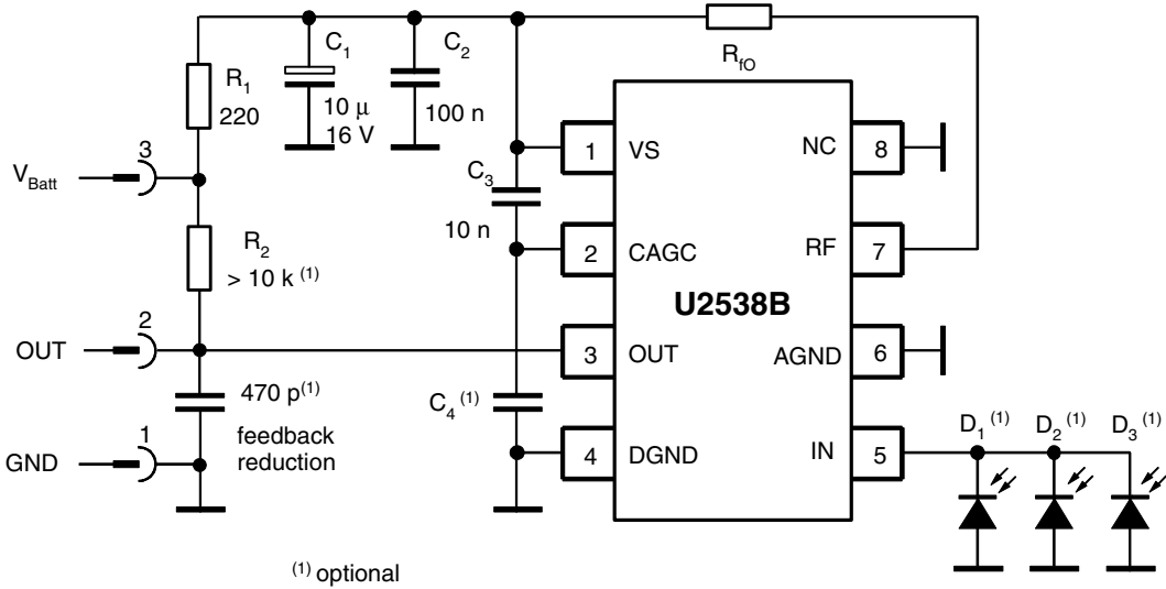
Figure 6-2. Application Circuit
